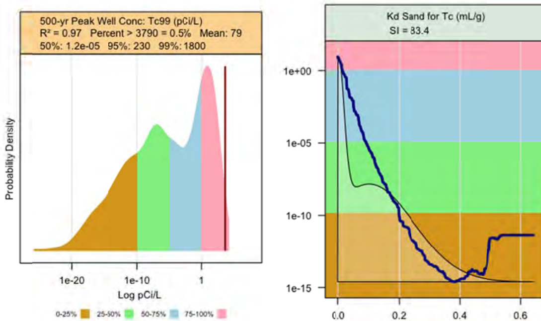
Figure 7. Partial dependence plot for peak ^{99}\text{Tc} groundwater concentration, assuming waste at 3 m.
